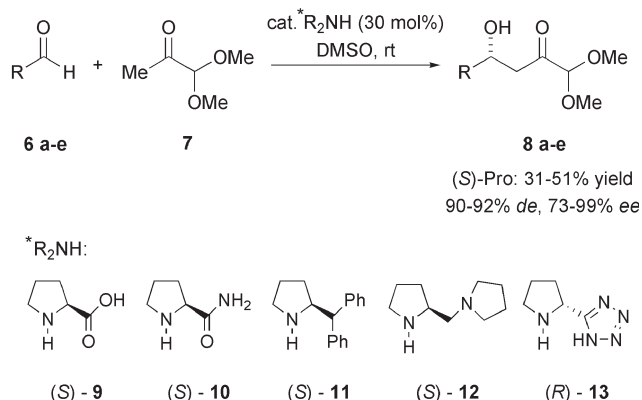
Scheme 1 Organocatalysed aldol reactions of the pyruvic aldehyde dimethyl acetal 7 with aldehydes 6 .
